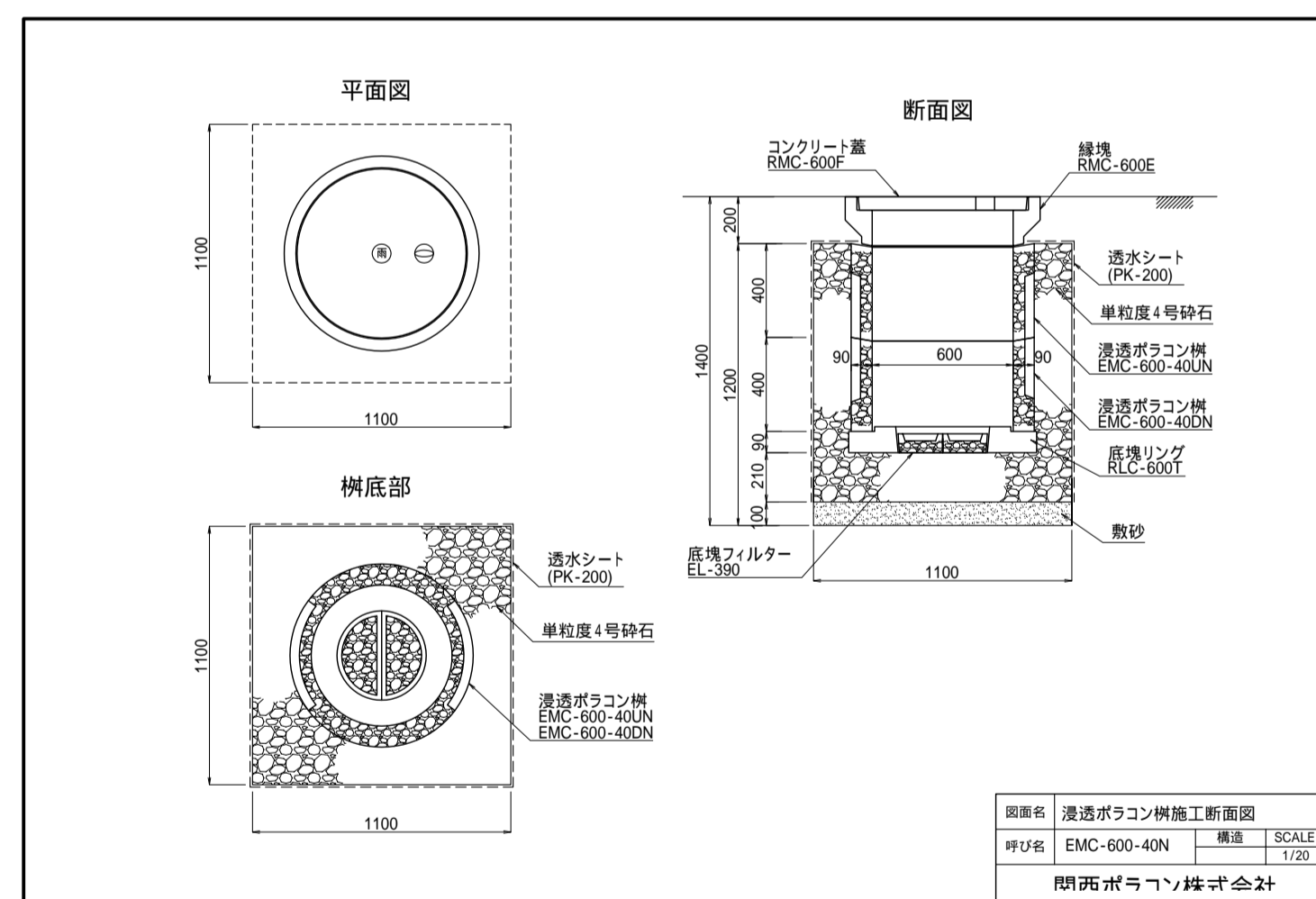
EMC-600-40N
