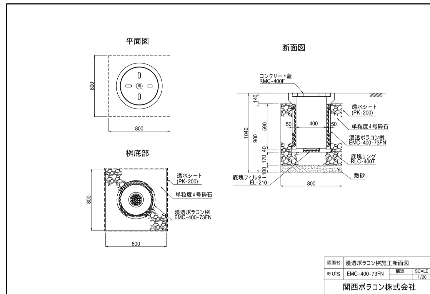
EMC-400-73N
