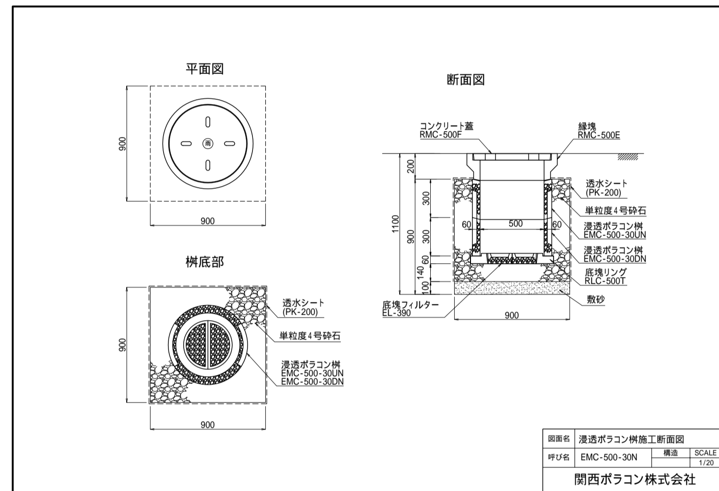
EMC-500-30N
