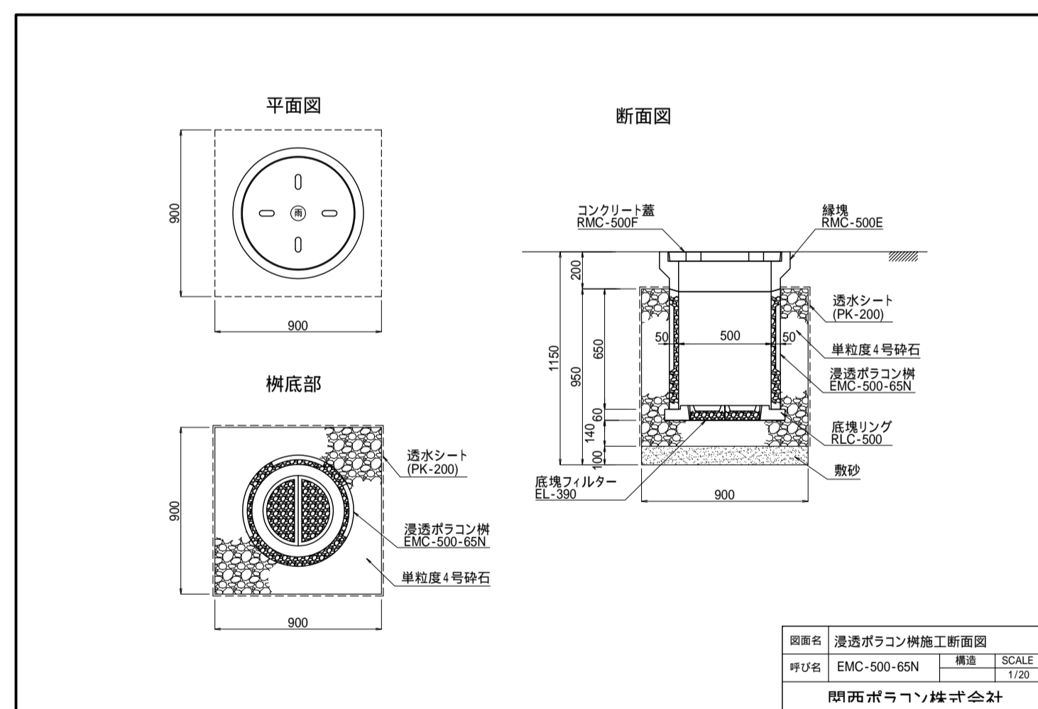
EMC-500-65N
